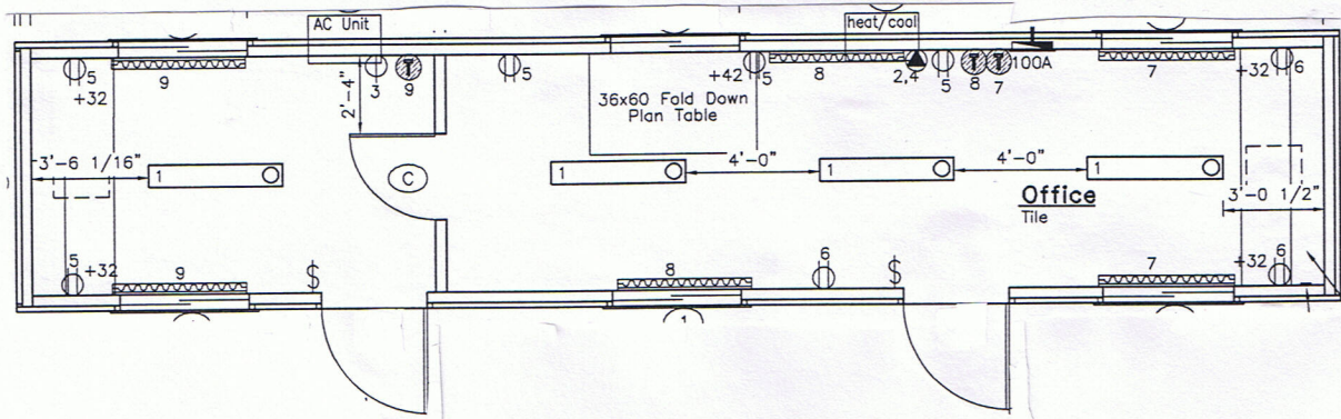
8' x 40' OFFICE CONTAINER
